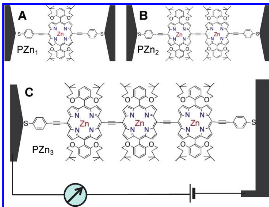
Figure 1. Schematic describing STM break junction-based single molecule conductance measurements for the \alpha,\omega -di[(4'-thiophenyl)ethynyl]-terminated PZn_n compounds (dithiol- PZn_1 (A), dithiol- PZn_2 (B), and dithiol- PZn_3 (C)) examined in this study.
