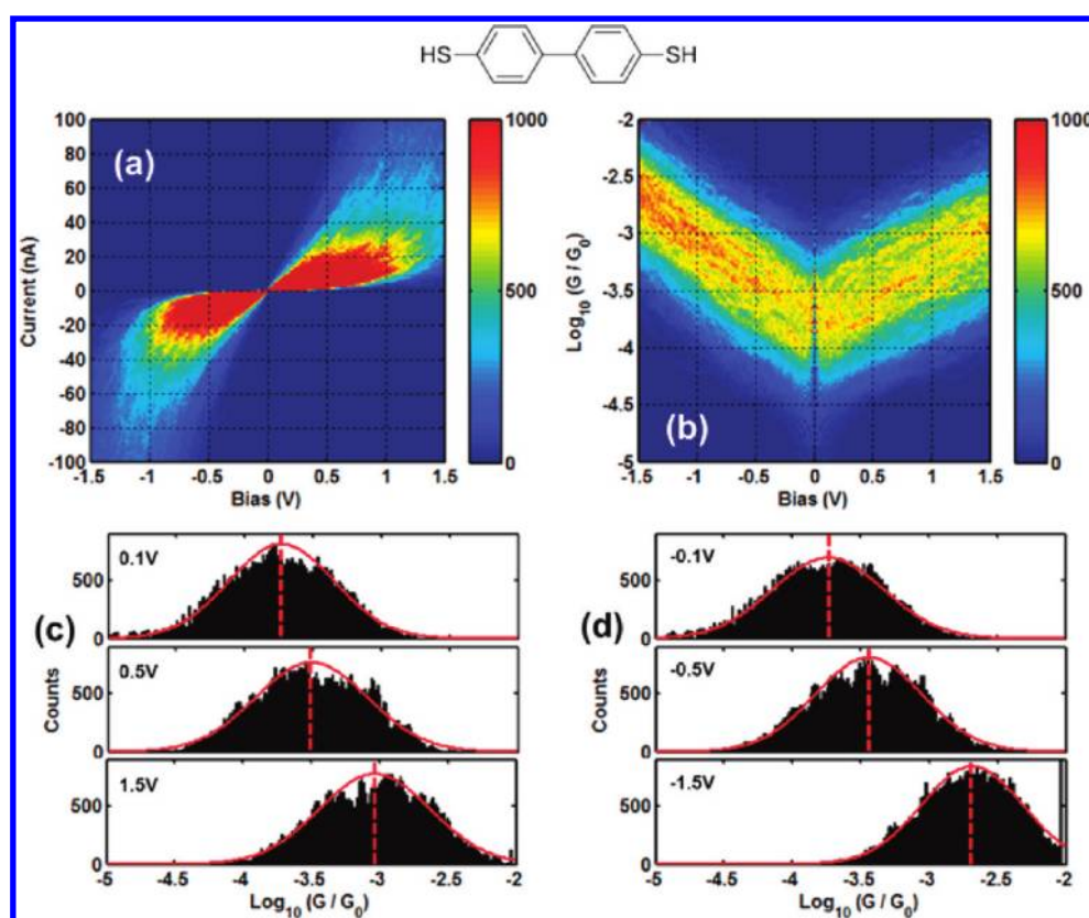
Figure 3. I-V (a) and G-V (b) histograms for biphenyldithiol consisting of 1258 curves. (c) 1-D conductance histogram at different positive (c) and negative (d) bias voltages.
