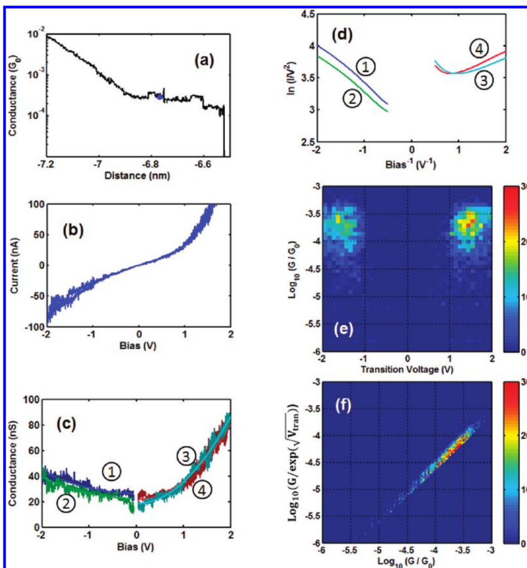
Figure 4. Transition voltage spectroscopy (TVS) and histograms. (a) Typical conductance trace for an H-junction of C8. (b) An I-V curve recorded at the position marked by a blue spot in (a). (c) G-V curves and fittings (smooth curves with lighter colors). (d) Corresponding TVS with colors matching the G-V curves in (c). (e) A 2-D histogram showing the distribution of transition voltage vs low-bias conductance. (f) Correlation between contact conductance vs low-bias conductance.
