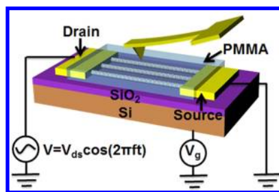
Figure 1. Schematic illustration of the experimental setup for scanning Joule expansion microscopy (SJEM) imaging of a SWNT device that incorporates several parallel, aligned tubes. The device consists of three terminals: two metal pads that contact the SWNTs to serve as the drain (alternating voltage) and source (grounded), and a third (doped silicon substrate) that serves as a gate. A layer of poly(methyl methacrylate) (PMMA) covers the device to protect the SWNTs and amplify the thermo-mechanical expansion caused by the Joule heating. An AFM probe operating in contact mode detects this expansion.
