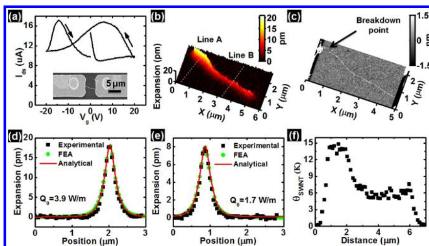
Figure 3. (a) Transfer curve of a single SWNT measured at V_{ds} = 3 V (DC voltage); the response indicates metallic behavior. The inset shows a scanning electron microscope (SEM) image of the device. (b) SJEM image of the same device, collected with V_{ds} = 3 V, f = 30 kHz, and PMMA thickness \sim 120 nm. (c) Topographical AFM image of the SWNT collected after removing the PMMA and operating the device at high bias in air. The location of degradation (breakdown point) coincides with that of the highest thermal expansion signal. (d,e) Expansion signal profiles (black solid square) along the cross sections marked by dotted lines A and B in (b), respectively. Green solid circles and red lines represent results from 2D FEA and analytical models, respectively, in which the power density, Q_0 , serves as a fitting parameter: Q_0 = 3.9 \mu\text{W}/\mu\text{m} for line A and Q_0 = 1.7 \mu\text{W}/\mu\text{m} for line B. (f) Calculated temperature distribution along the SWNT based on the SJEM measurement.
