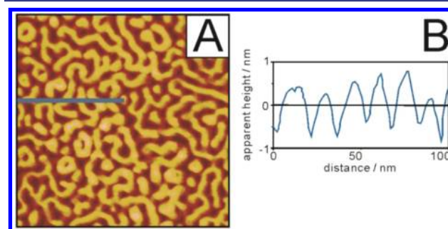
Figure 3. (A) STM image recorded in decane, size 200 nm \times 200 nm and (B) typical cross section of an Au(111) surface after 1000 s exposure to a 0.5 mM OPE1/1.0 mM TBAF solution in THF (for further details see SI) and cross-section analysis of the blue line.
