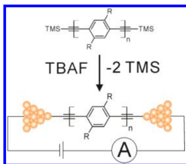
Scheme 2. Molecules Studied in This Work
