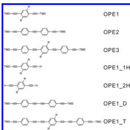
Scheme 2. Molecules Studied in This Work
