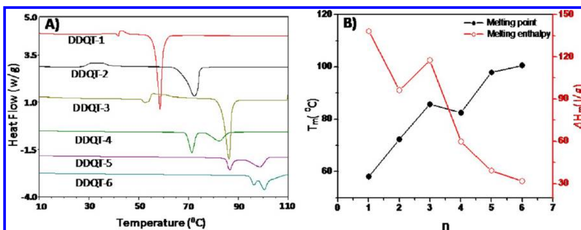
Figure 5. (A) DSC heating process with a rate of 10 °C/min and (B) melting points and melting enthalpies ( \Delta H_m ), from the oligothiophene powder samples measured by DSC as a function of oligomer number.
