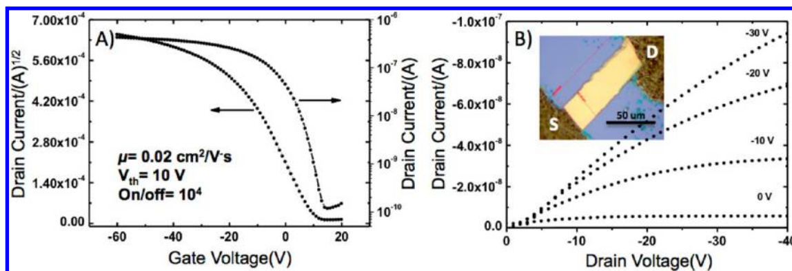
Figure 10. (A) The transfer/square root of current characteristics and (B) output characteristics of a DDQT-3 single crystal transistor. Inset: single crystal transistor of DDQT-3 on Si/SiO 2 (300 nm) with carbon paste as top-contact source-drain electrodes.
