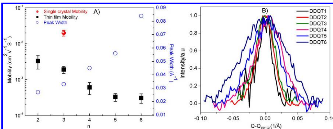
Figure 12. (A) Thin-film carrier mobilities of oligothiophenes (black squares) and in-plane peak widths (open circles) as a function of oligomer length. A single crystal transistor of DDQT-3 is shown in red circles. (B) Overlay of the evolution of the peak width at |q| = 1.0 \text{ \AA}^{-1} that can be found in the oligothiophene diffraction pattern series. The data shows a significant decrease in crystalline order with increasing oligomer length.
