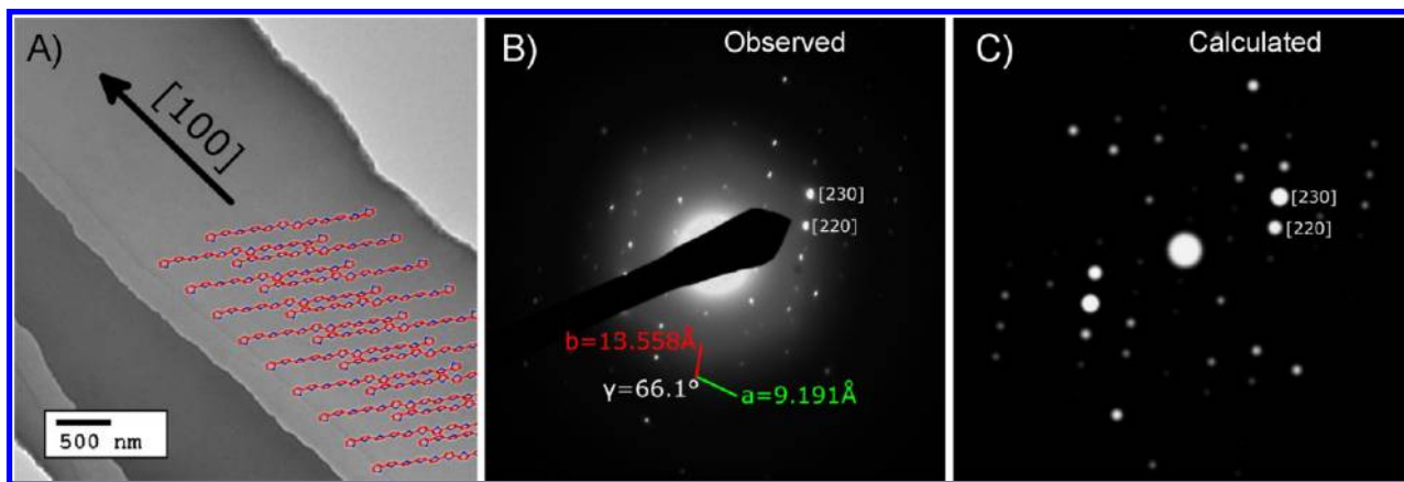
Figure 11. (A) TEM of a DDQT-3 single crystal with elucidated molecular packing overlay, (B) the corresponding diffraction image with measured a - and b -unit cell dimensions, and (C) the “calculated” electron diffraction pattern generated from the bulk structure refinement data using CrystalMaker software, Ltd.
