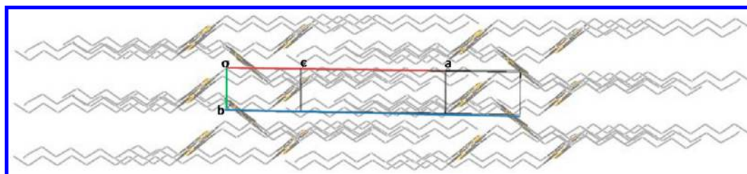
Figure 7. Herringbone packing and alkyl chain interdigitation of DDQT-2. Hydrogens were omitted for clarity.
