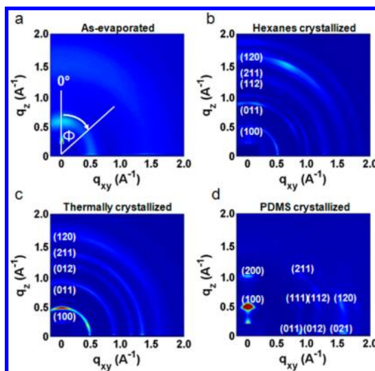
Figure 2. Indexed grazing-incidence X-ray diffraction images of as-evaporated (a), hexanes-vapor annealed (b), thermally annealed (c), and PDMS-crystallized (d) HBC films on HMDS-treated SiO 2 . Azimuthal anisotropy of diffracted intensity indicates preferential orientation of HBC.
