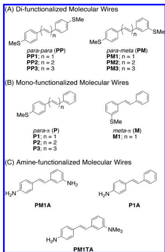
Figure 1. Chemical structures of trans -stilbene and all- trans -oligoene molecular wires: (A) difunctionalized series, having only para -positioned linker groups (PP n ) or a mixture of para and meta linkers (PM n ); (B) monofunctionalized wires P n and M1 contain either one meta or one para linker. (C) Stilbene derivatives end-functionalized with primary and tertiary amines.
