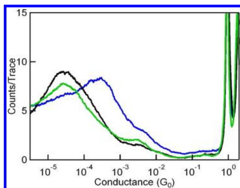
Figure 4. Log-binned conductance histograms of amine-functionalized stilbene molecular wires: para - meta PMIA (blue), para - \pi PIA (green), and methylated para - meta PMITA (black) were generated from 5000 individual conductance traces.
