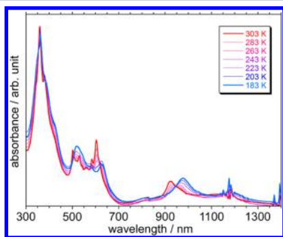
Figure 5. Electronic absorption spectra of 3b in \text{CH}_2\text{Cl}_2 ( 3.6 \times 10^{-5} M) for different temperatures.
