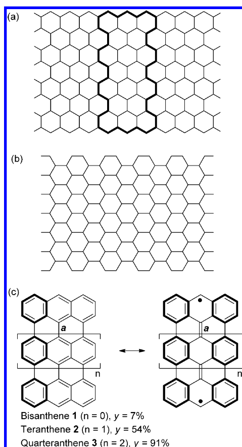
Figure 1. Chemical structure of GNRs and anthenes. (a) Zigzag-edged GNR (15.4 Å ribbon width). The bold line represents a quarteranthenene (3) skeleton. (b) Armchair-edged GNR (14.5 Å ribbon width). (c) Resonance structure of anthenes. The amount of singlet biradical character ( y ) was calculated at the CASSCF(2,2)/6-31G level. The six-membered rings depicted by bold lines represent the Clar sextets.
