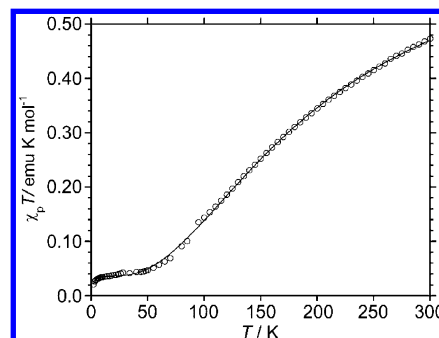
Figure 4. \chi T - T plot for the powdered 3a . The measured data are plotted as open circles. The line is the theoretical curve calculated using the alternating Heisenberg chain model with parameters of 2J_{\text{intra}}/k_B = -347 K, 2J_{\text{inter}}/k_B = 2\alpha J_{\text{intra}}/k_B = -151 K ( \alpha = 0.436 ), impurity spin contamination = 5.0%, g = 2.002 , and diamagnetic susceptibility = -894.5 \times 10^{-6} emu/mol.
