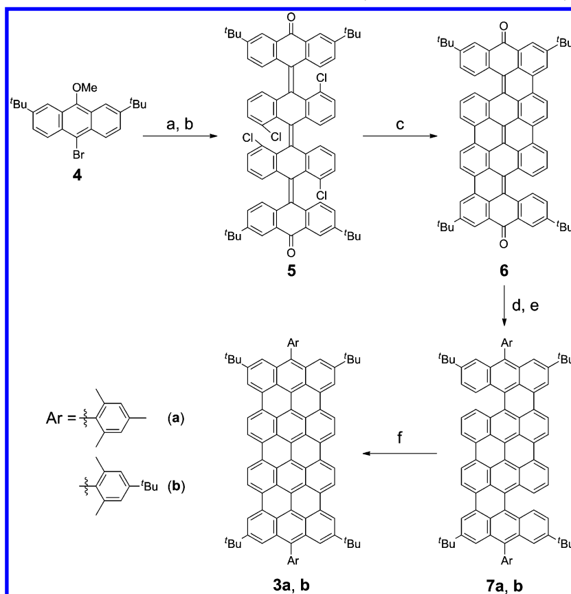
Scheme 1. Stepwise Synthetic Route to Quarteranthenes 3a (Ar = Mesityl) and 3b (Ar = 4- tert -Butyl- m -xylyl) a
