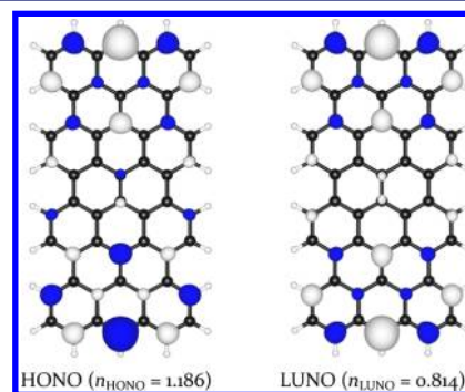
Figure 7. Isosurface maps and occupation numbers of HONO and LUNO obtained from the ground-state electron density calculated at the CASSCF(8,8)/6-31G* level of approximation. White/blue meshes represent the isosurfaces with contour values of +0.03/-0.03 au.
