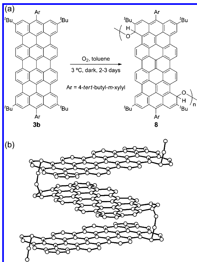
Figure 8. (a) Reaction of 3b with oxygen. The most dominant Clar structure is drawn for 11 on the basis of the HOMA analysis. (b) X-ray structure of 8 . Ar, t\text{Bu} groups, and H atoms are omitted for clarity.
