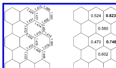
Figure 3. (Left) Mean bond lengths (Å) in the main core ring of 3a , and (right) HOMA values of 3a .
