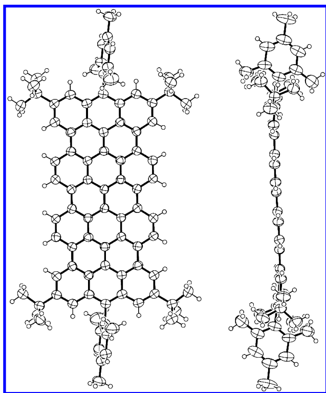
Figure 2. ORTEP drawings of 3a at the 50% probability level: (left) top view and (right) side view.
