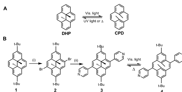
Figure 1. (A) DHP/CPD system. (B) Synthesis of 3. Reagents and conditions: (i) NBS, DMF/ \text{CCl}_4 ; (ii) 4-pyridinylboronic acid, Pd( \text{PPh}_3 ) 4 , \text{Na}_2\text{CO}_3 , THF/ \text{H}_2\text{O} , reflux, 29%.
