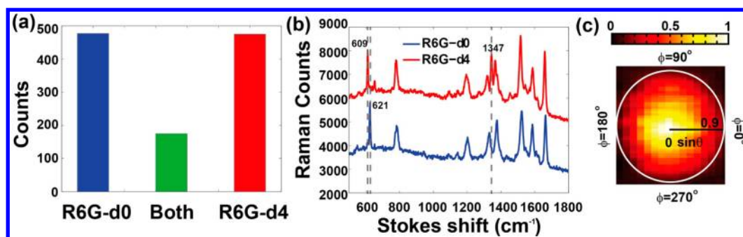
Figure 3. Experimental results of SMSERS using the optical antenna chip we introduce. (a) Histogram of single molecule level events: R6G-d0 molecule (blue), both R6G-d0 and R6G-d4 molecules (green), and R6G-d4 molecule (red). (b) Representative Raman spectra of R6G-d0 and R6G-d4 single molecule level events. The R6G-d4 spectrum is shifted in the vertical direction by 2000 counts for display purposes. (c) Measured far-field emission pattern of 620 \text{cm}^{-1} Raman line of single molecule R6G-d0 event. The pattern is normalized by the maximum emitted signals. \theta and \phi are defined in Figure 1.
