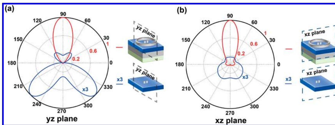
Figure 2. Calculated far-field radiation power intensity patterns for device we introduce (red curves) and basic optical antenna design (blue curves). Simulations performed at a wavelength of \lambda = 550.2 nm ( 620 \text{cm}^{-1} Raman line with excitation at \lambda = 532 nm). The radiation power patterns are normalized by the peak power radiated by the optical antenna design we introduce. For comparison purposes, the results for the basic optical antennas (blue curves) have been multiplied by 3\times . (a) Calculated radiation patterns on yz plane. (b) Calculated radiation patterns on xz plane.
