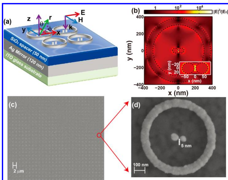
Figure 1. Optical antenna chip. (a) Schematic of optical antenna chip for SMSERS. Each antenna consists of pair of Ag particles (5 nm gap) surrounded by an Ag ring, all on a SiO 2 spacer layer on a Ag mirror on ITO-coated glass. Ag rings have inner and outer radii of 300 and 380 nm, respectively. Ag particles and rings are 40 nm thick (in z -direction). Ag particles are rods (70 nm long and 60 nm wide in x - and y -directions) with rounded ends (30 nm radius). Periodicities of the antennas in x and y -directions are both 2 μm. (b) Profile of the simulated intensities of electric field at the wavelength of \lambda=532 nm on xy plane and 20 nm above the top surface of SiO 2 spacer. Intensities of electric field are normalized by that of the incident wave. Polarization and propagation direction of incident wave are given in Figure 1a. Dashed lines indicate outlines of silver ring and particle pair. Inset: intensities of electric field around particle pair. (c,d) Scanning electron microscope images of optical antenna chip. Overall extent of optical antenna array is 100 μm × 100 μm. Inner and outer radii of silver rings are 300 and 380 nm, respectively. Left-hand rod of optical antenna is 80 nm long and 70 nm wide. Right-hand rod of optical antenna is 68 nm long and 62 nm wide.
