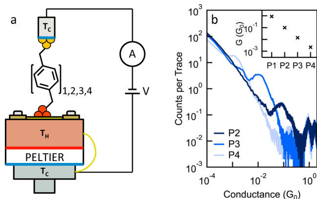
Figure 1. (a) Schematic of the STM-BJ setup representing thermoelectric measurement of P1–P4 . (b) Conductance histograms of P2–P4 obtained during the thermoelectric measurement. The bin size is 10^{-4} G_0 . Inset: Conductance plotted as a function of number of phenyls in the molecular backbone.
