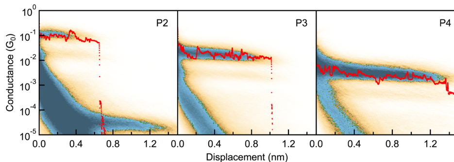
Figure 2. Two-dimensional conductance histograms of P2–P4 . A representative conductance trace for each molecule is shown as a superimposed dotted lines. The bins have a width of 0.008 nm along the displacement axis and 100/decade along the conductance axis. The molecular plateau between 10^{-5} and 10^{-4} G_0 in the 2D histogram for P2 is due to the dimer molecule formed in situ.
