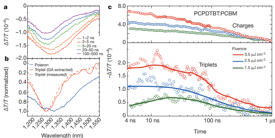
Figure 4 | Triplet and charge kinetics for PCPDTBT blends. a , Temporal evolution of the transient absorption spectrum for PCPDTBT:ICBA, excited with an excitation fluence of 2 μJ cm -2 . Temporal slices are averaged over the indicated time periods and smoothed. A blueshift of the spectra from a peak at 1,300 nm to 1,275 nm can be seen over the first 100 ns. b , Triplet spectrum extracted from the genetic algorithm (GA) analysis (solid red line) and that measured by doping a PCPDTBT thin film with a triplet sensitizer (dashed red line). The blue line shows the charge spectrum as measured 50 ps after
