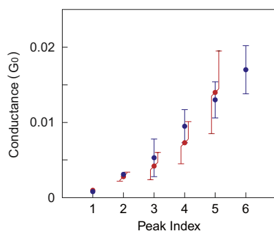
Figure 4. Positions of conductance peaks obtained from histograms measured in Ar (red dots) and in solution (blue dots), respectively. (For interpretation of the references to color in this figure legend, the reader is referred to the web version of this article.)
