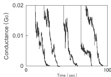
Figure 2. Examples of the conductance trace of the Au/BDTA/Au junction.
