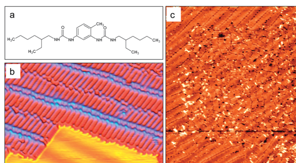
Fig. 1 (a) Scheme of the EHUT molecule. (b) 20 \times 12.3 \text{ nm}^2 topographic image of an ordered monolayer of EHUT on Au(111) ( V_s = -500 \text{ mV} , I_t = 570 \text{ pA} , T = 77 \text{ K} ). Every continuous object corresponds to one single molecule. The bare gold substrate underneath the molecules can be seen at the bottom of the image. 14 (c) 50 \times 60 \text{ nm}^2 topographic image of an initially ordered monolayer of EHUT where a 40 \times 40 \text{ nm}^2 area was disturbed by a previous scan at -50 \text{ mV} and 2 \text{ nA} . Many bonds in the layers are broken due to the tip interactions leading to sub-units such as short dimer-rows, few assembled molecules and single molecules randomly oriented with various conformations.
