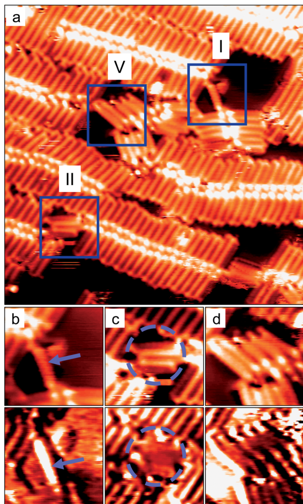
Fig. 4 (a) The supramolecular monolayer was disturbed by the z -distance and voltage pulses resulting in a few isolated molecules and patches of molecules disconnected from the main layer ( 20 \times 20 \text{ nm}^2 , V_s = -500 \text{ mV} , I_t = 380 \text{ pA} ). Three different regions are highlighted. (b)–(d) Zoom of STM images ( 4 \times 4 \text{ nm}^2 ) of isolated patches of 1, 2 and 5 EHUT molecules corresponding to the frames I, II and V in (a). The upper row exhibits the topography images while the lower row shows the corresponding differential conductance images ( dI/dV maps).
