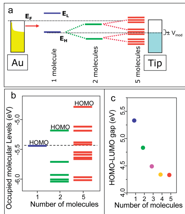
Fig. 5 (a) Illustration of the possible interpretation of the bright and dark contrast seen in the dI/dV maps of Fig. 4 showing a variation of the HOMO–LUMO gap as a function of coupled molecules. (b) Gaussian calculation of the splitting of the HOMO level of EHUT as a function of the number of molecules associated together via H-bonding. The scale is related to the vacuum level. (c) Evolution of the HOMO–LUMO gap for the same configuration of molecules. For more than 4 molecules, the gap remains almost constant.
