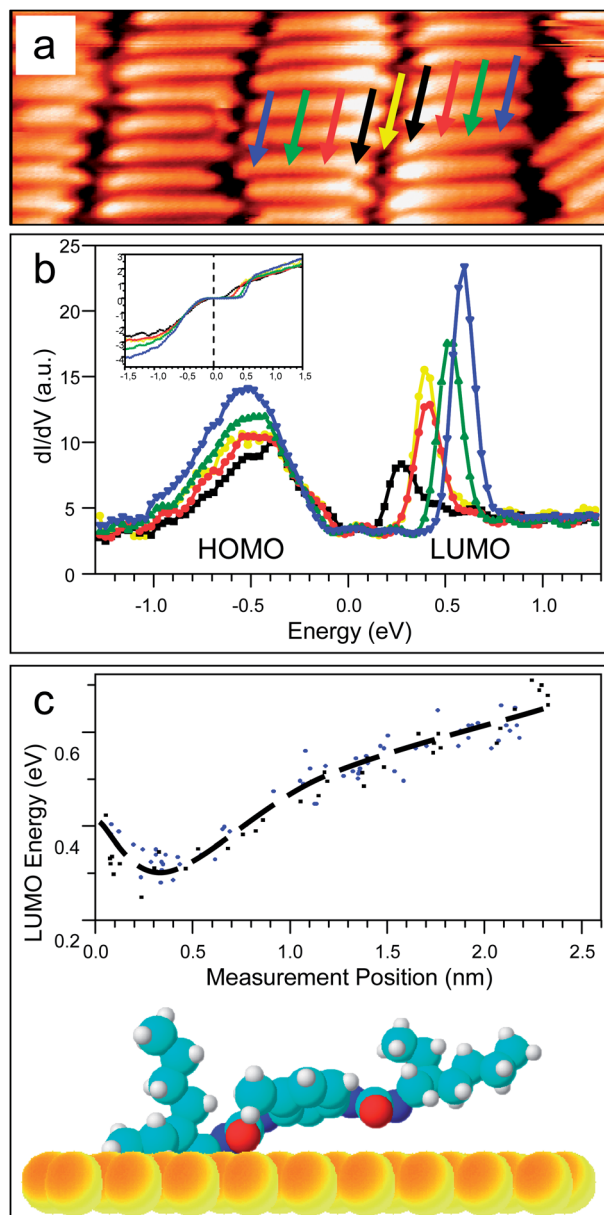
Fig. 2 (a) STM image of a monolayer of EHUT ( 3.5 \times 10 \text{ nm}^2 , V_s = -0.5 \text{ V} , I_t = 1.2 \text{ nA} , 77 \text{ K} ). Arrows represent the positions along the EHUT molecules where spectroscopy measurements were taken. The corresponding dI/dV spectra (and I(V) in the inset) according to the color code are represented in (b). (c) Representation of the energy of the LUMO state along the molecule (conformation calculated in ref. 20) measured as a function of the distance to the zipper line (yellow arrow in (a)). The dashed line was drawn to guide the eye.
