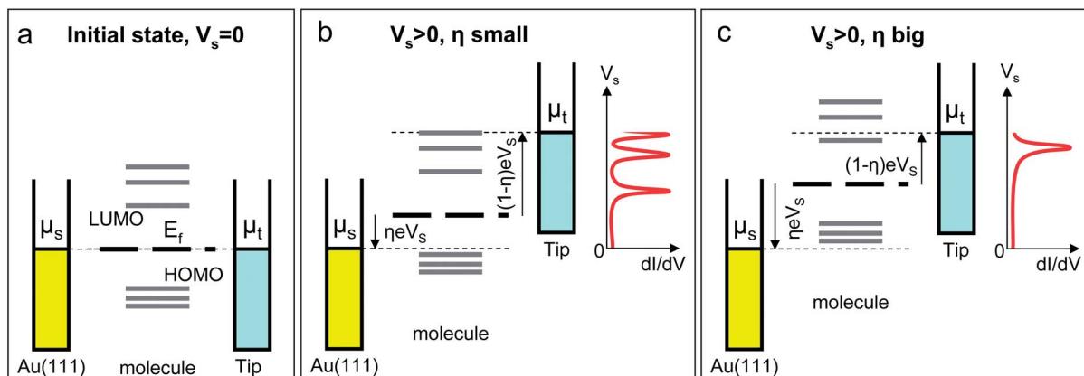
Fig. 3 Illustration of the charging effect relating the shift of the position of the LUMO peaks to the parameter \eta (see text). (a) Bias voltage is zero and the Fermi levels of the substrate, molecule and tip are aligned within the junction. In (b), \eta is small (close to zero), representing the case of strong hybridization of the molecule and the substrate. The resulting shift of the Fermi level of the molecule is also small and when increasing the bias voltage the first LUMO peak appears close to the actual value. (c) represents the case of a rather weak adhesion between the substrate and the molecule corresponding to \eta close to 1. Thus, the charging effect is large and the measured electronic levels appear at higher values of the bias voltage. This apparent shift of the LUMO level is seen in the dI/dV versus V_s curves of Fig. 2.
