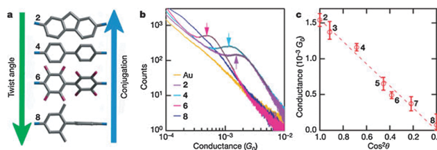
Fig. 13 Dependence of single-molecule junction conductances on molecular conformation. Reprinted by permission from Nature Nanotechnology (L. Venkataraman, J. E. Klare, C. Nuckolls, M. S. Hybertsen and M. L. Steigerwald, Nature , 2006, 442 , 904–907), Copyright (2006). 142
