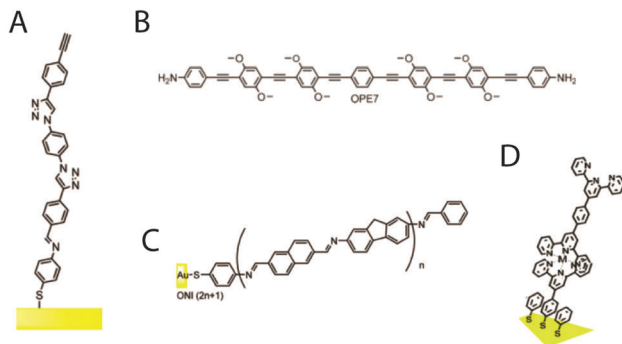
Fig. 11 (A) Oligophenylene triazole (OPT) synthesized by click chemistry, (B) oligo( p -phenylene ethylenes): OPE7, (C) oligofluorene imine (ONI) and (D) a metal containing molecular wire as examples for typical molecules for single-molecule electronics. 174
